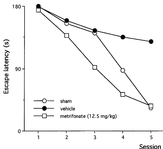
Fig. 1. Effects of metrifonate on performance in the Morris' water maze task in basal forebrain-lesioned rats. Metrifonate was administered orally 30 min before each trial. Each point represents the mean.
